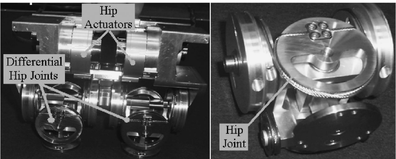
Figure 7. Mechanical realization and torque transmission cable rooting of the differential hip joints.
