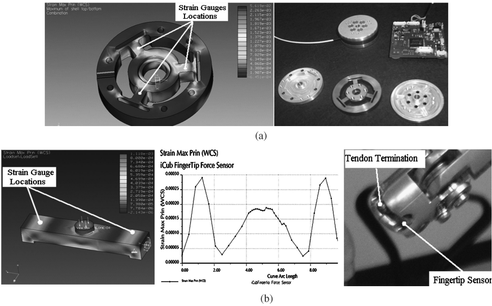
Figure 14. (a) The 6-d.o.f. F/T sensor and (b) the tendon force fingertip sensor.
