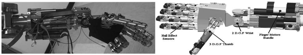
Figure 12. The iCub hand and the forearm section.
