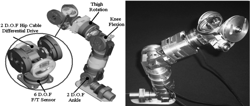
Figure 6. Mechanical realization of the iCub leg.
